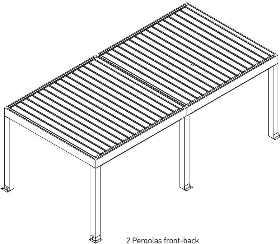
2 Pergolas front-back
