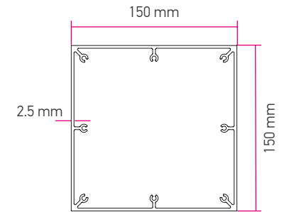
3 column 150X150
