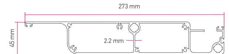
5 panel 273X45
