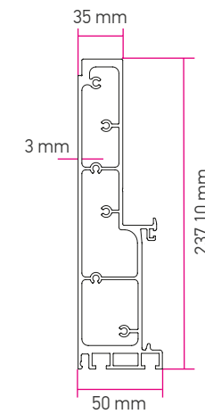
1 rafter 50X237
