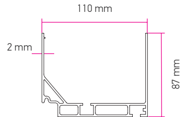
② perimetric gutter 110X87
