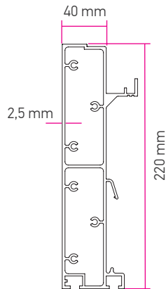
① rafter 40X220
