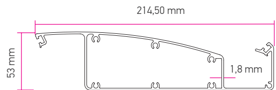
⑤ panel 214,5X53
