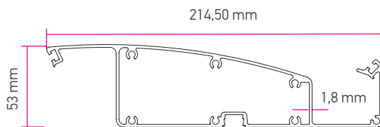
④ panel for LED lighting 214,5X53
