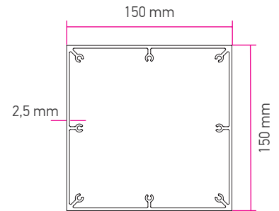
③ column 150X150
